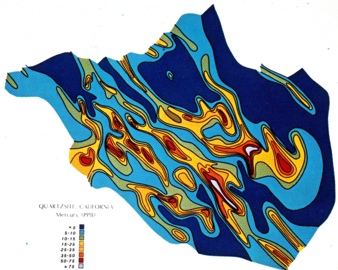
Mobile mercury associated with hydrothermal gold mineralization partially covered by gravel.
