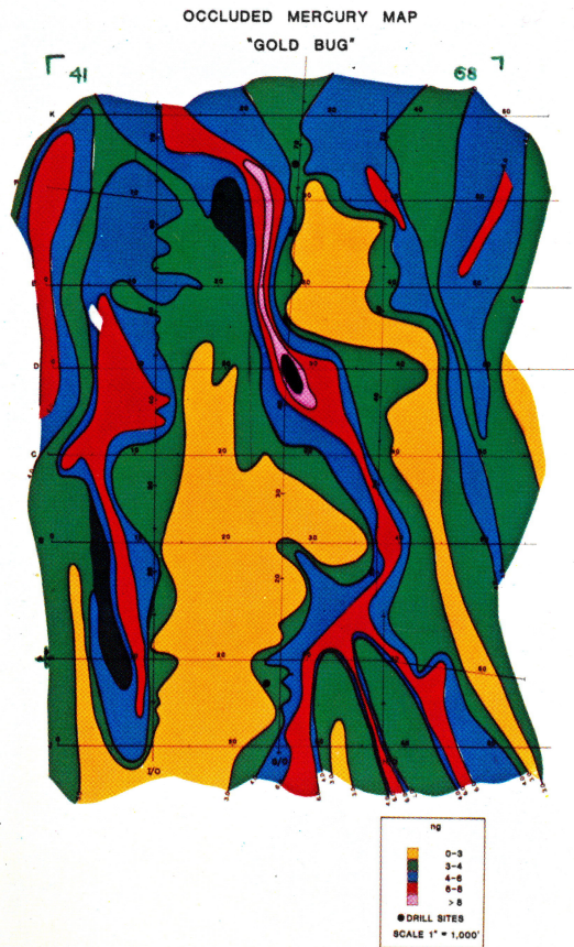
Mobile mercury over volcanic gold mineralization covered by gravel.
