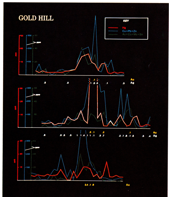
Correlation of mobile Hg with Au, Ag and other elements from Au vein in Appalachia.
