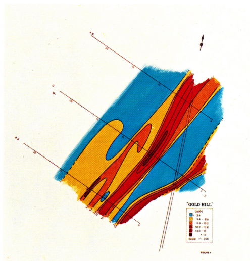
Mobile mercury association with Au vein in Appalachia.
