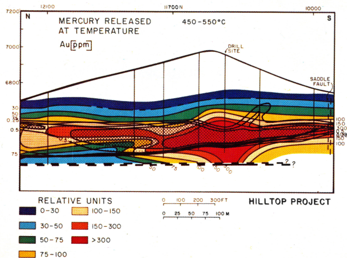
Vertical cross-section of mercury forms associated with gold mineralization.
