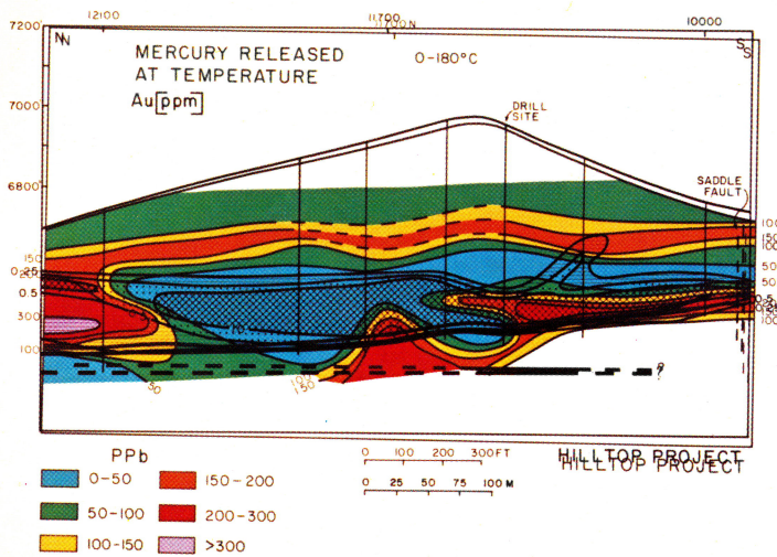
Vertical cross-section of mobile mercury analyzed from drill holes.
