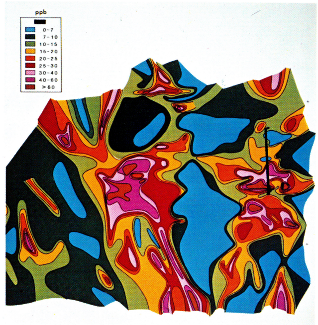
Surface expression of mobile Hg over Carlin type gold ore body.
