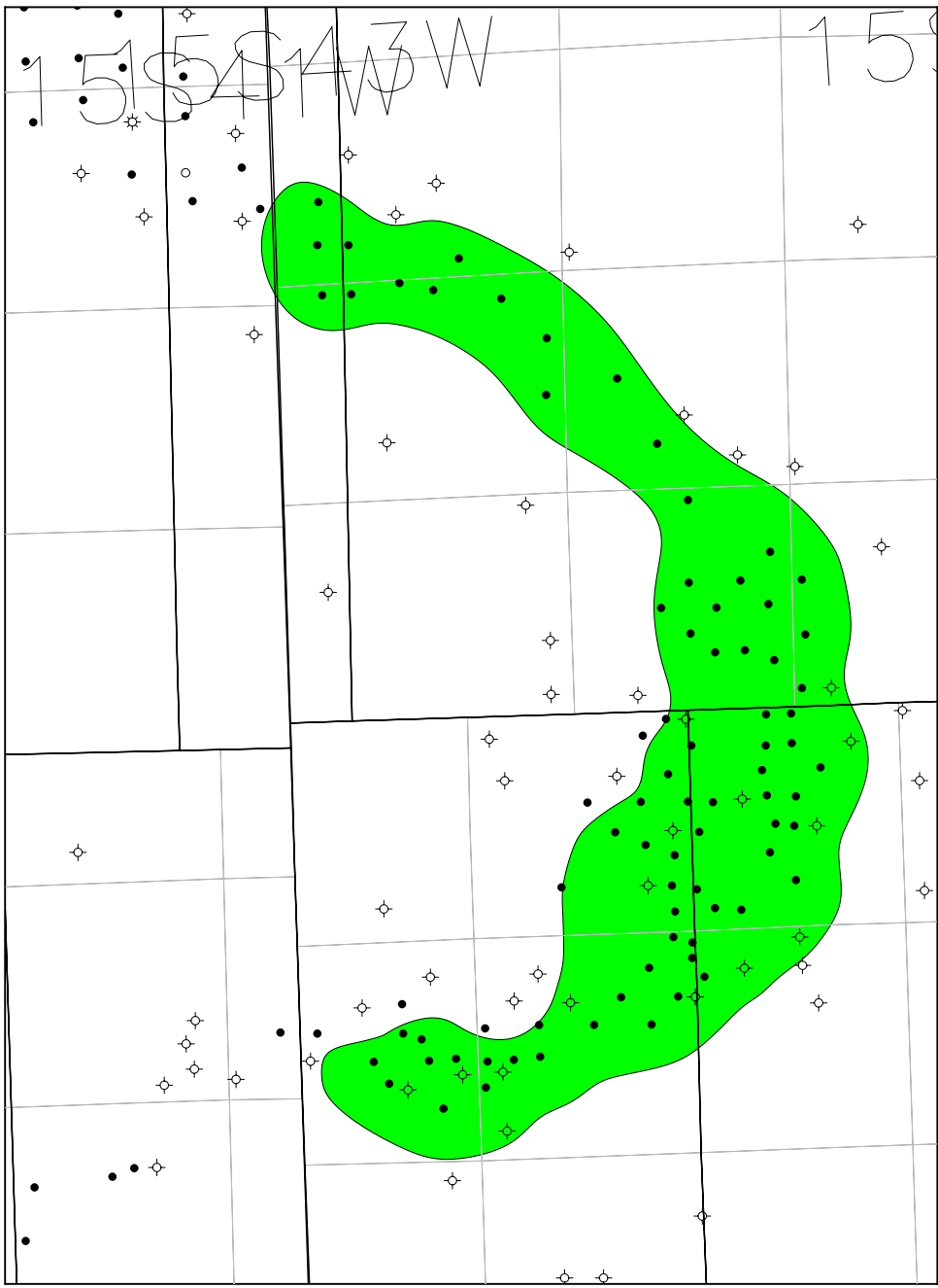
Stockholm Field Wallace & Greeley Cos., Kansas
