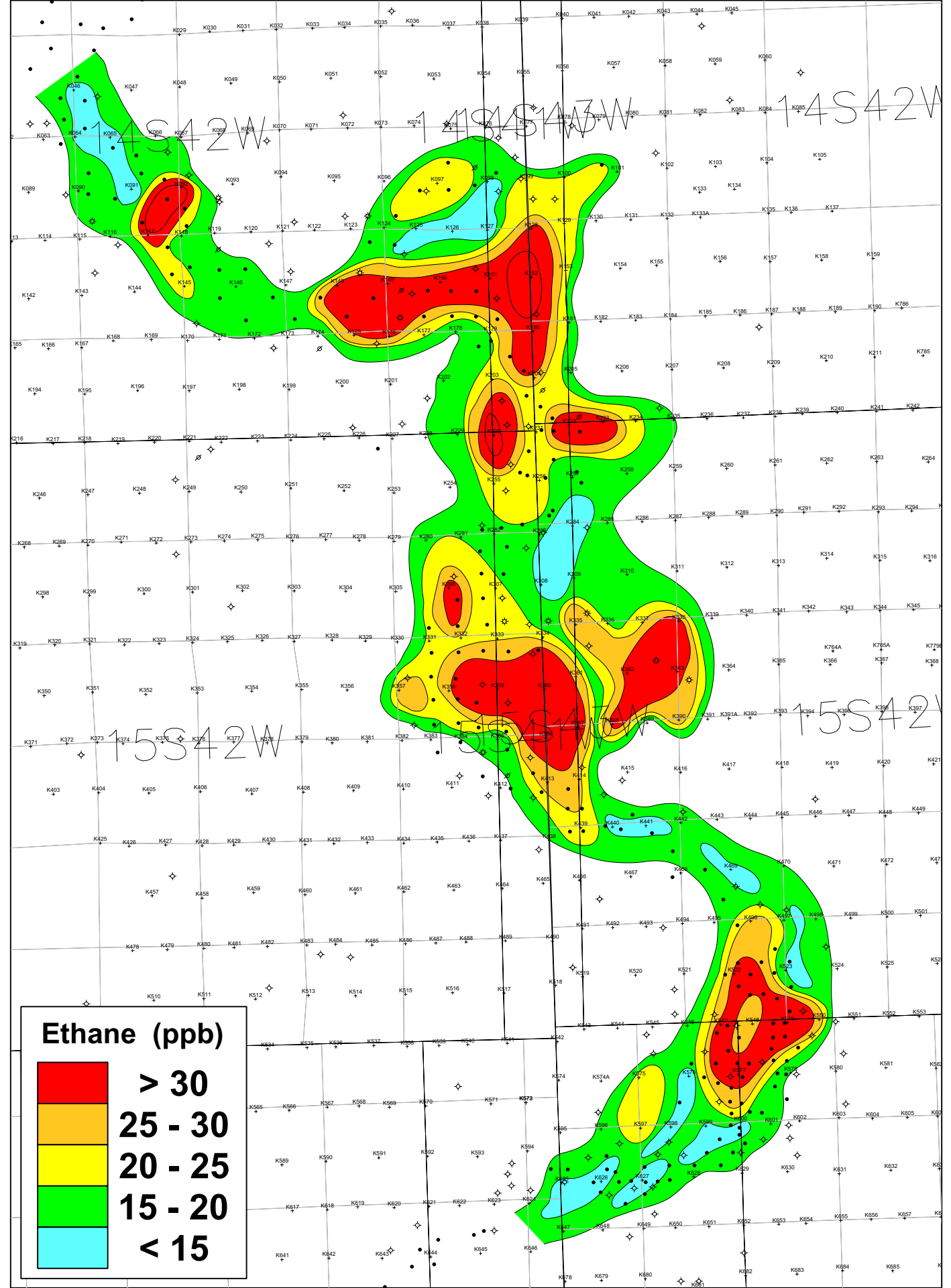
Soil Gas Survey Conducted - November 1987 Ethane Magnitude Contour Map
