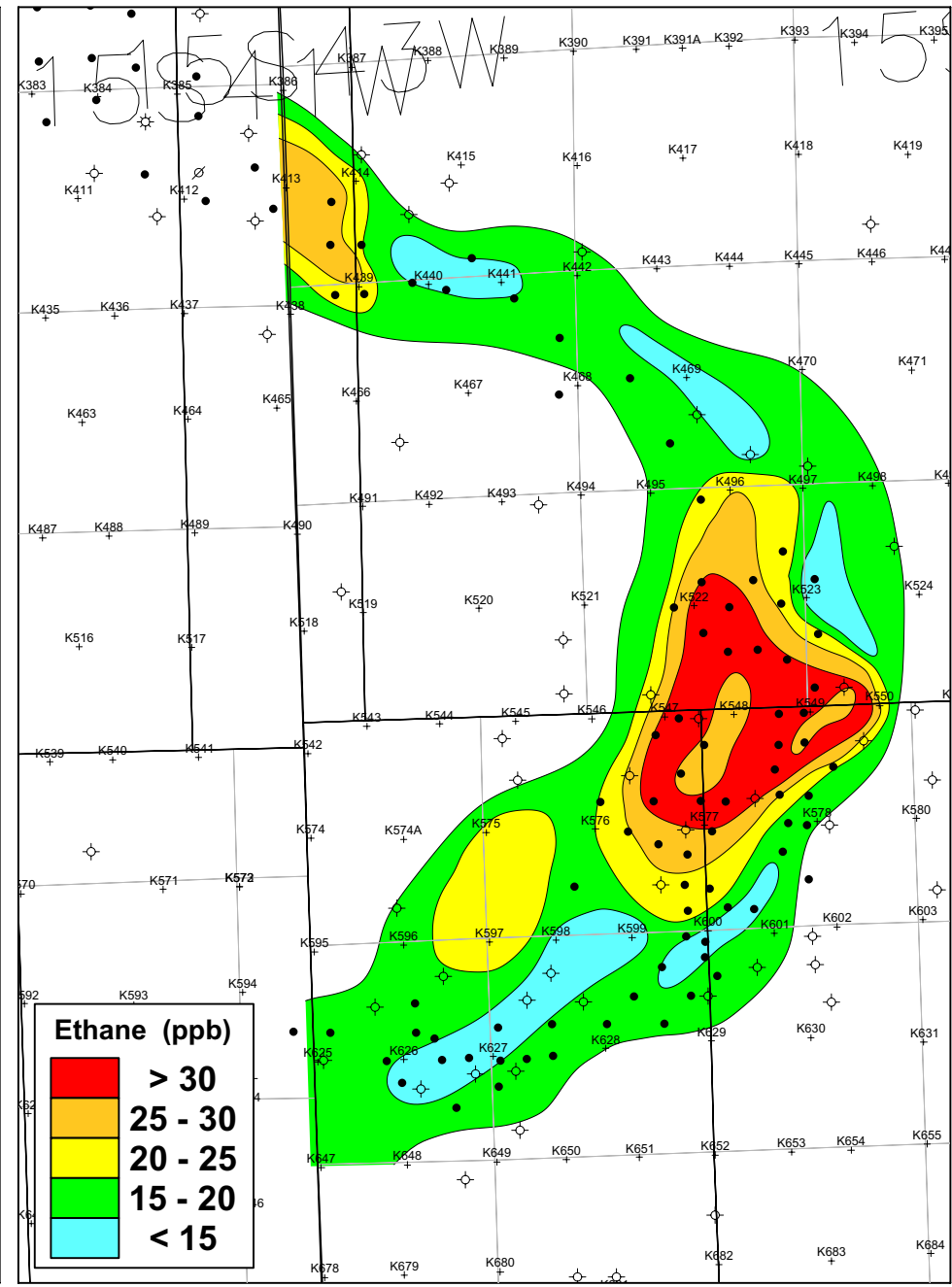
Stockholm Field Soil Gas Map - Ethane
