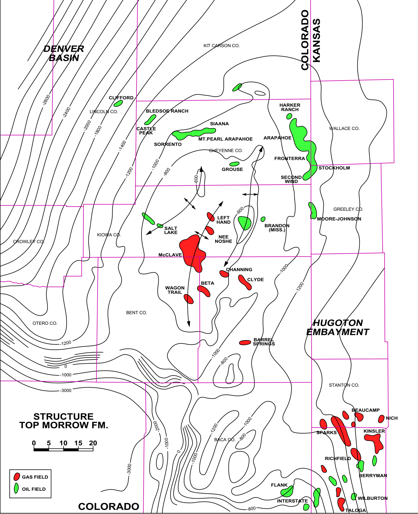
Structure Top Morrow FM.
