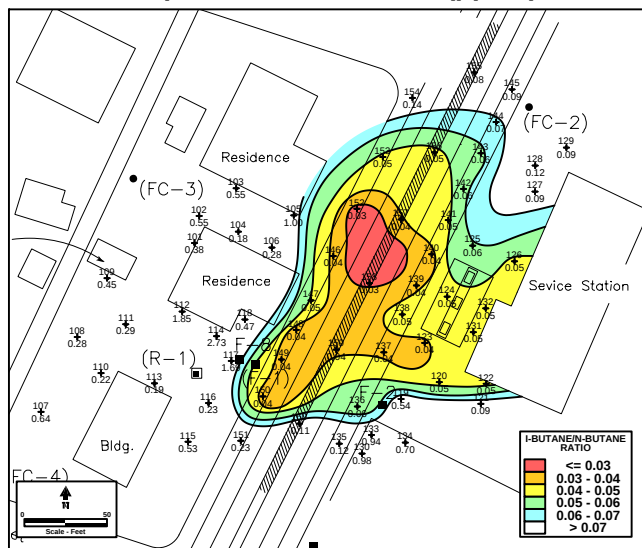
I-Butane/N-Butane Ratio
