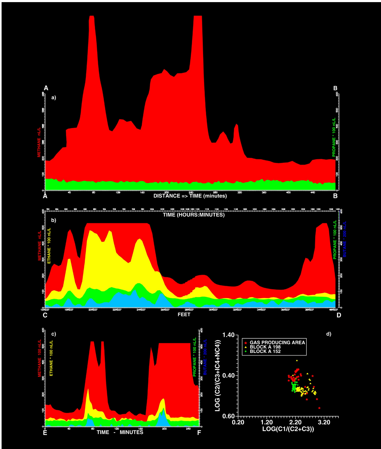
Fig. 5-34. Profile of dissolved hydrocarbon data from High Island sniffer survey; a) East-West Line A-B; b) South-North Line C-D; c) North-South-North Line E-F; d) Marine Compositional Crossplot for 1988 Sniffer Anomalies.
