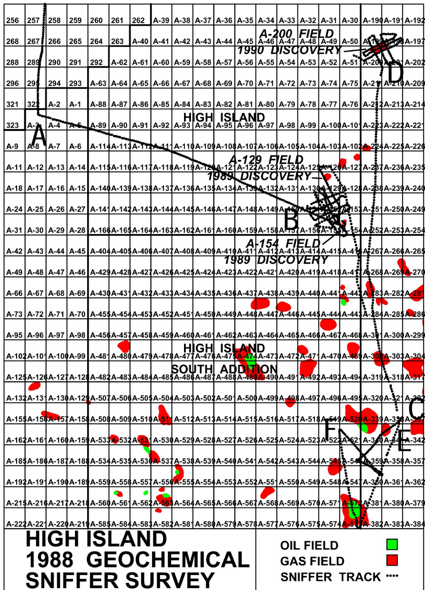
Fig. 5-33. a) High Island Geochemical Sniffer Track Map for 1988 Sniffer Survey; b) Marine Compositional Crossplot for 1988 Sniffer Anomalies.
