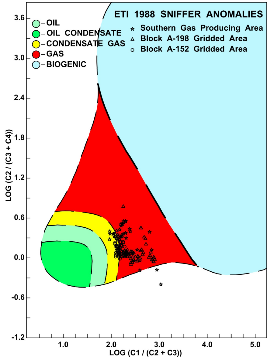
Fig. 5-33. a) High Island Geochemical Sniffer Track Map for 1988 Sniffer Survey; b) Marine Compositional Crossplot for 1988 Sniffer Anomalies.
