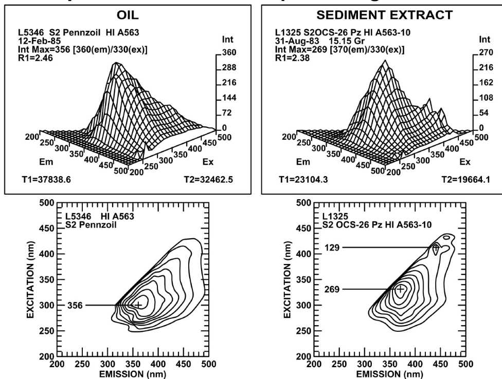
Fig. 5-28. Fluorograms of reservoir hydrocarbons and corresponding hydrocarbons extracted from sediments in the Gulf of Mexico. (Reproduced with permission from J. Brooks, GERG).
