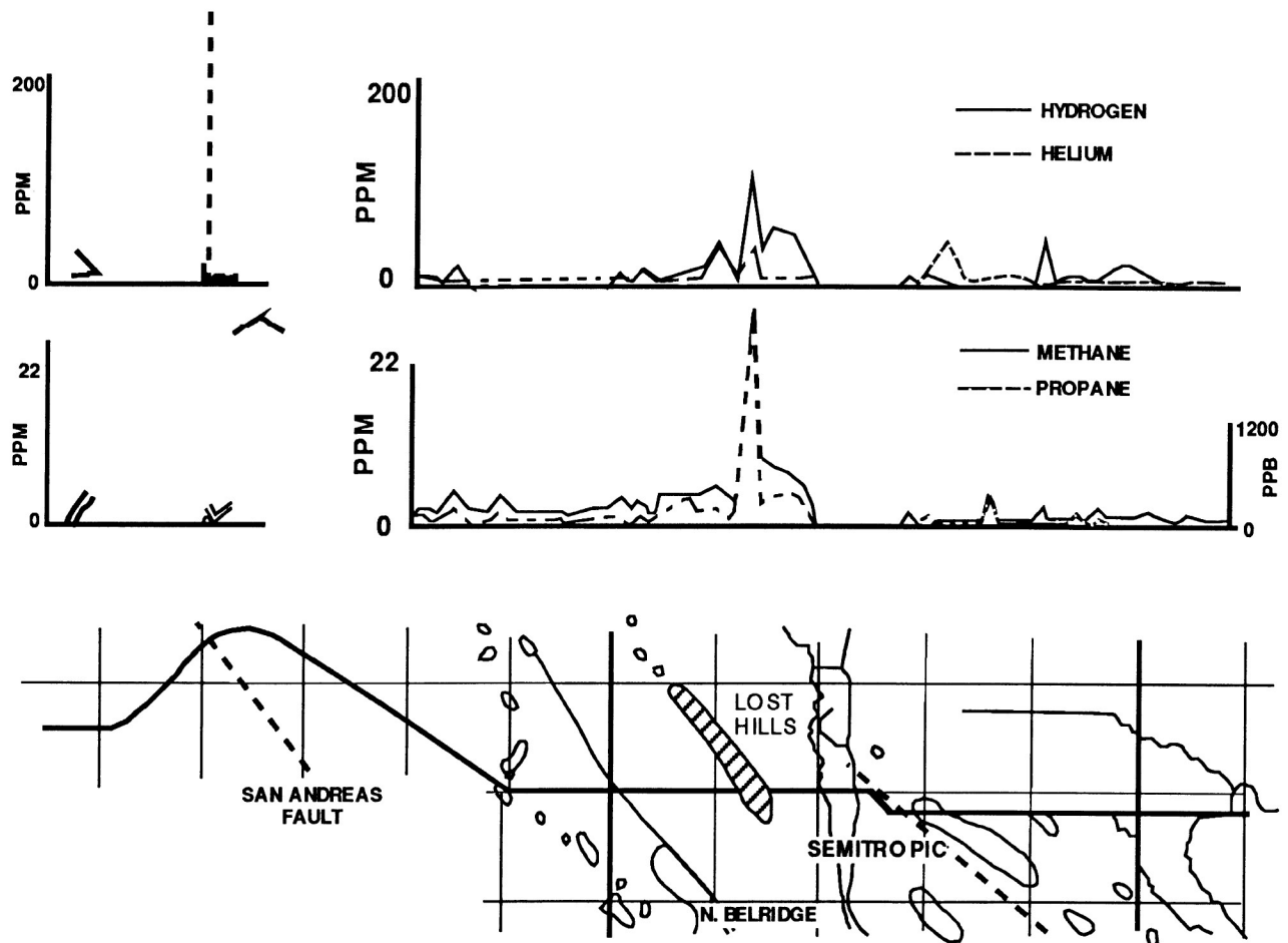
Fig. 5-12. Relation of near-surface gases to deep faults and oil fields along a traverse in the San Joaquin Valley, California (reproduced with permission from Jones and Drozd, 1983).
