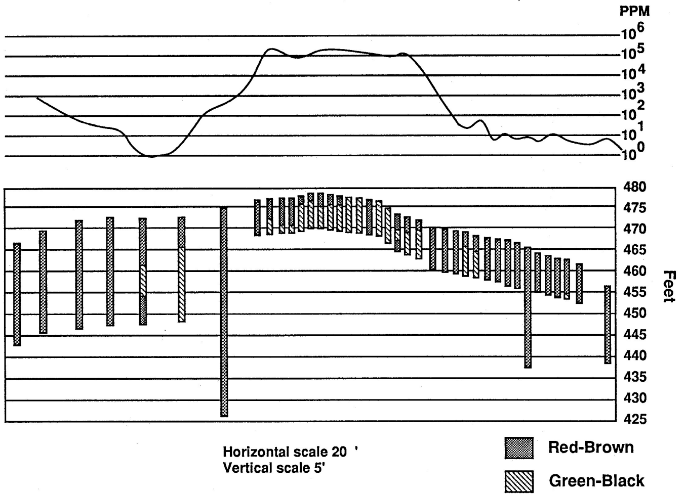
Fig. 5-11. Propane concentrations and soil colour of augered samples along a traverse of sample sites over an underground propane storage reservoir.
