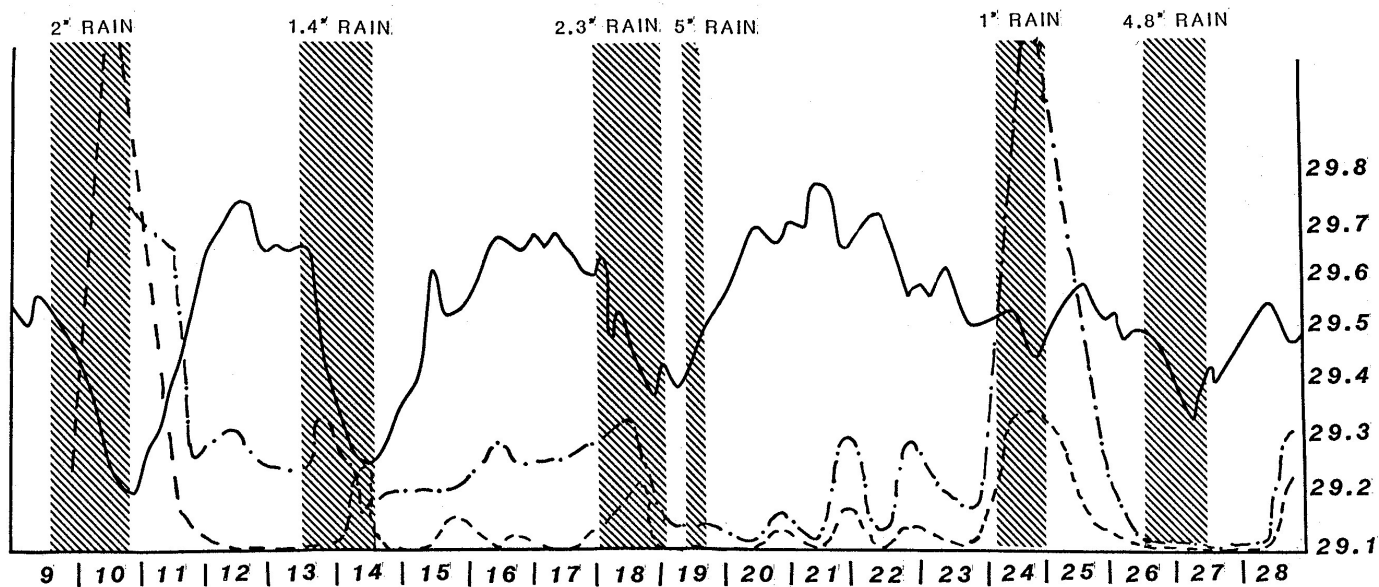
Fig. 5-10. Changes in flux of propane concentration (dashed lines) with barometric pressure (solid line) and rainfall (shaded bars) at two surface sample sites over an underground propane storage reservoir.
