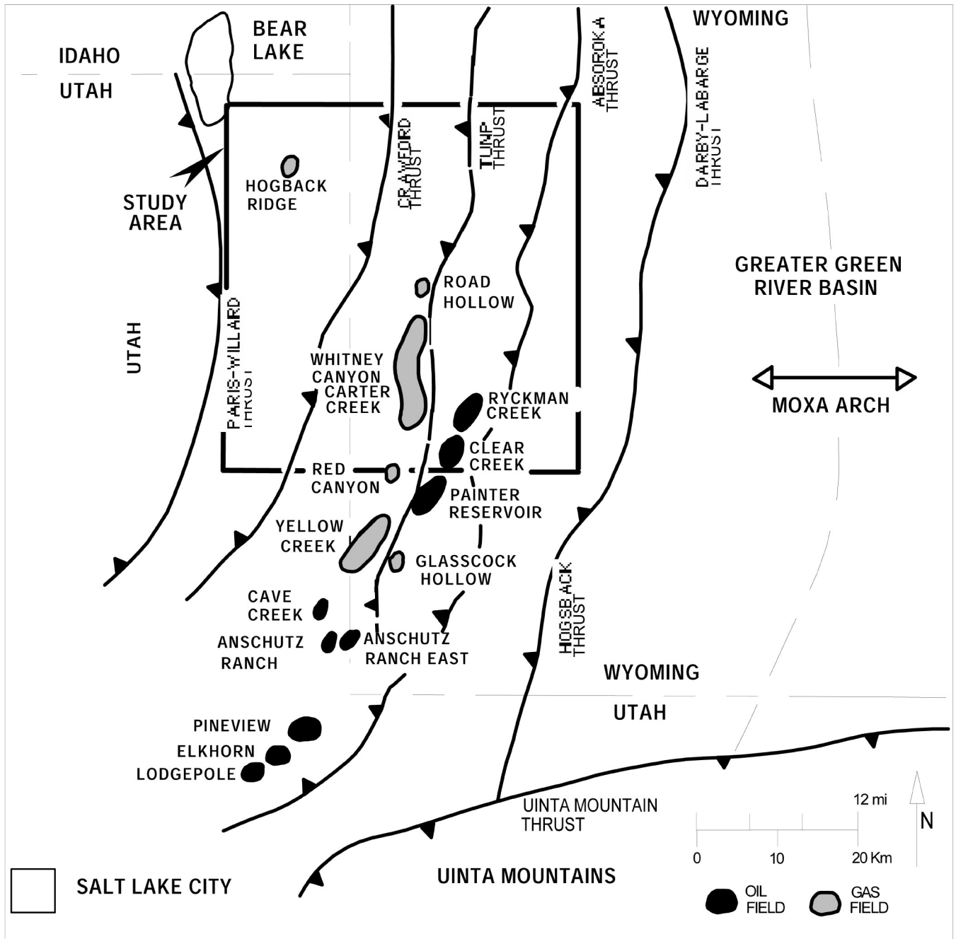
Fig. 5-43. Clear Creek, Ryckman Creek, and Whitney Canyon-Carter Creek Fields.
