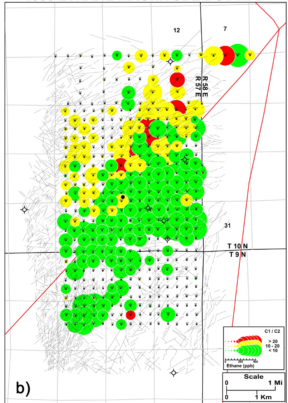
Fig. 5-42. Comparison of a) 1984 and b) 1985 Ethane Color Dot Maps, Illustrating Repeatability of Soil Gas Compositional Data.
