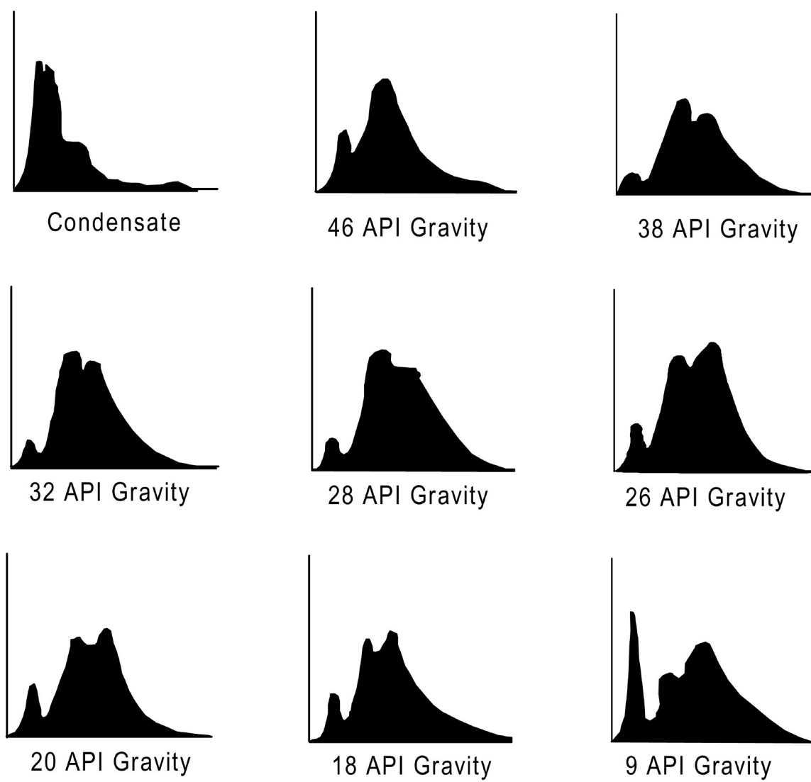
Fig. 5-27. Comparative fluorescence spectra of nine crude oils of different gravity (reproduced with permission from Purvis et al., 1977)
