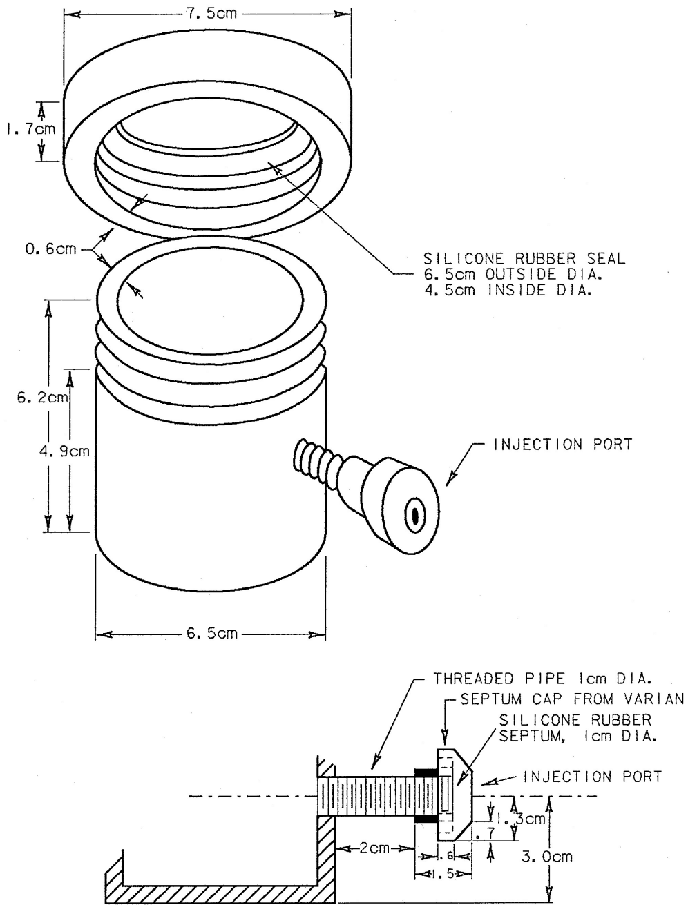
Fig. 5-25. Stainless steel disaggregation mill used in headspace analysis
