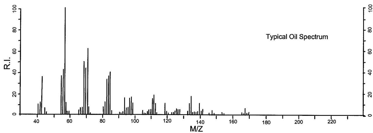
Fig. 5-17. Typical mass spectra of gas and oil, R. Klusman personal communication.
