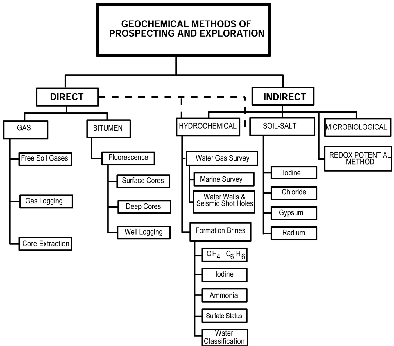
Fig. 5-6. Geochemical methods of prospecting for petroleum and natural gas (reproduced with permission from Kartsev et al., 1959).
