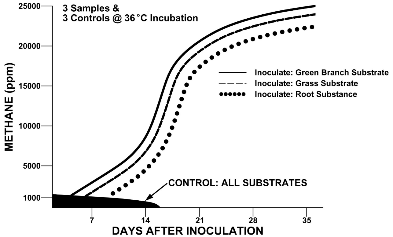
Fig. 5-5. Anaerobic microbial evolution of CH 4 upon decomposition of various organic substrates (reproduced with permission from Janezic, 1979)
