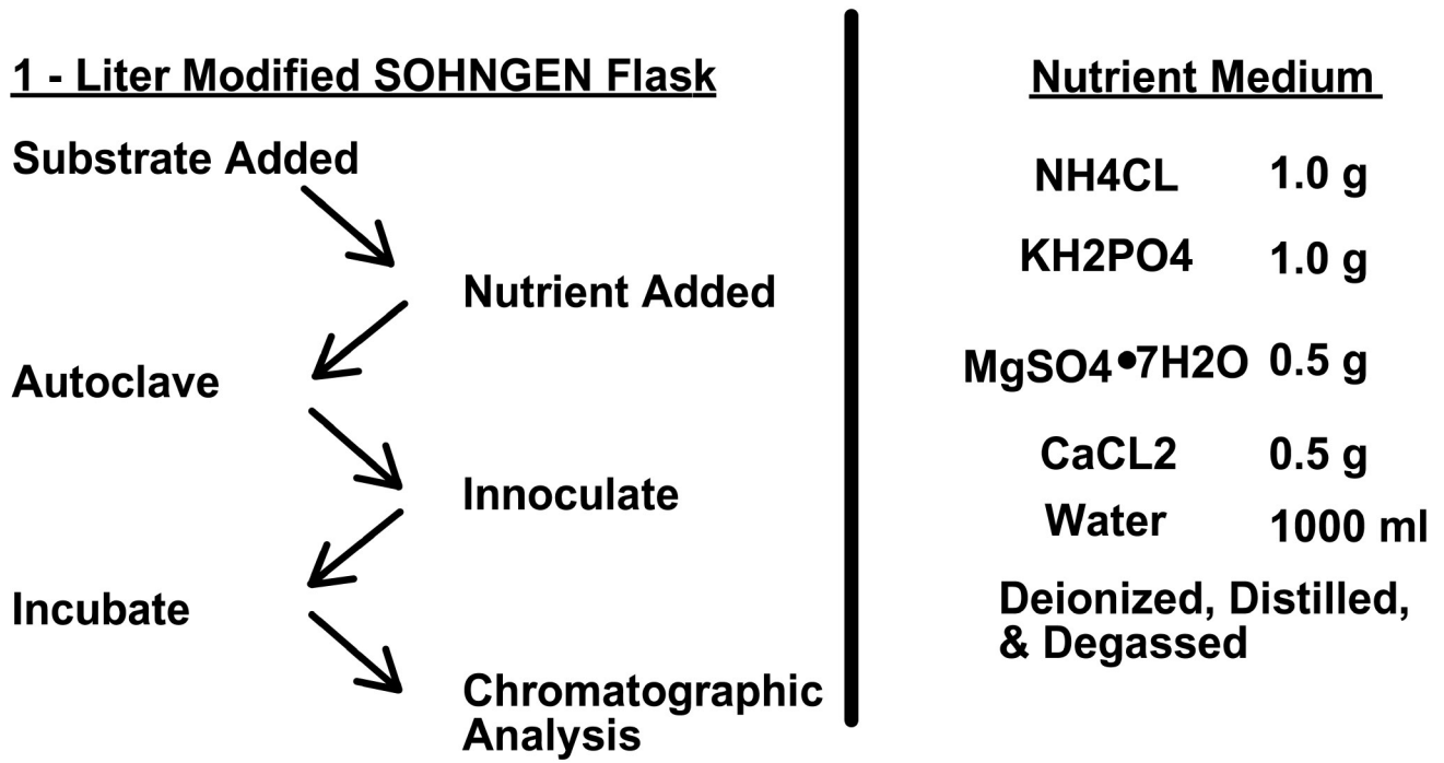
Fig. 5-4. Experimental scheme for anaerobic decomposition of natural organic matter (from Kim and Douglas, 1972).
