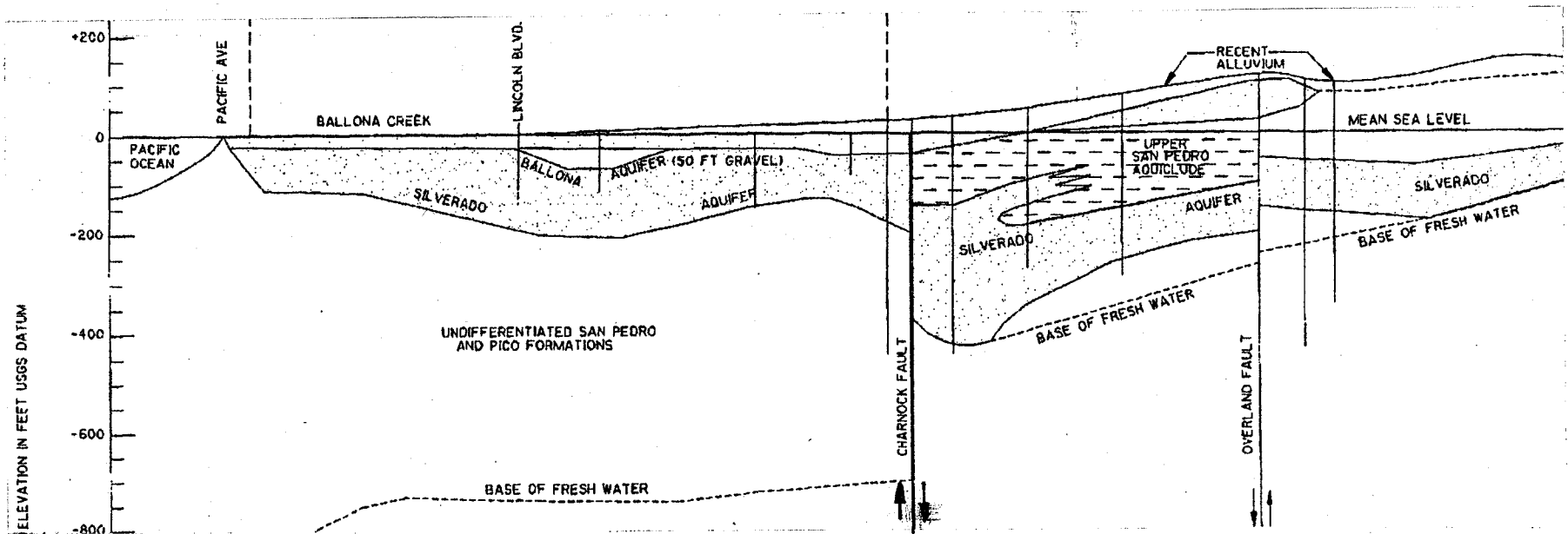
Figure 7. Generalized E-W Hydrogeologic Cross Section (Modified after Cal. Dept. Wtr. Res., 1961 & CDM, 1998)
